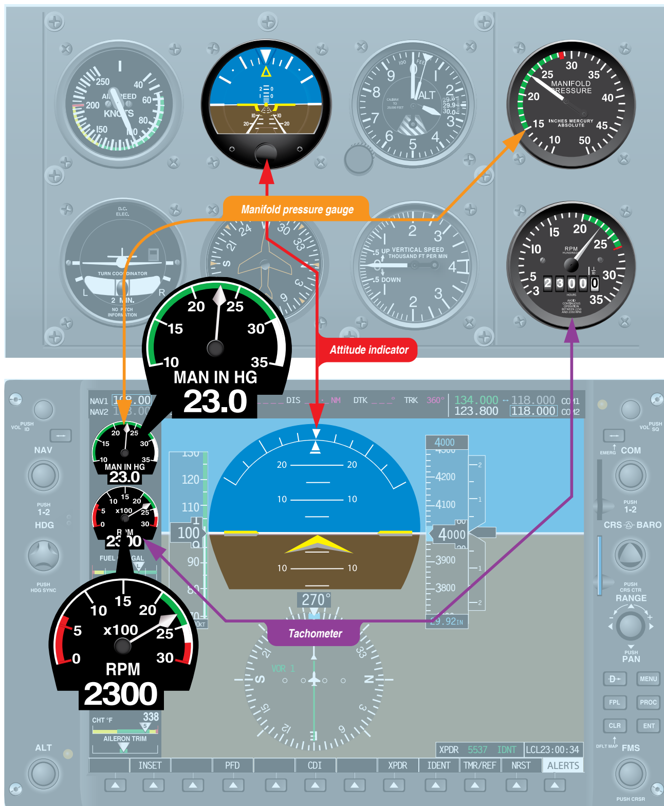
Figure 3-20. Control instruments.
